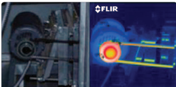
Misaligned Belts
